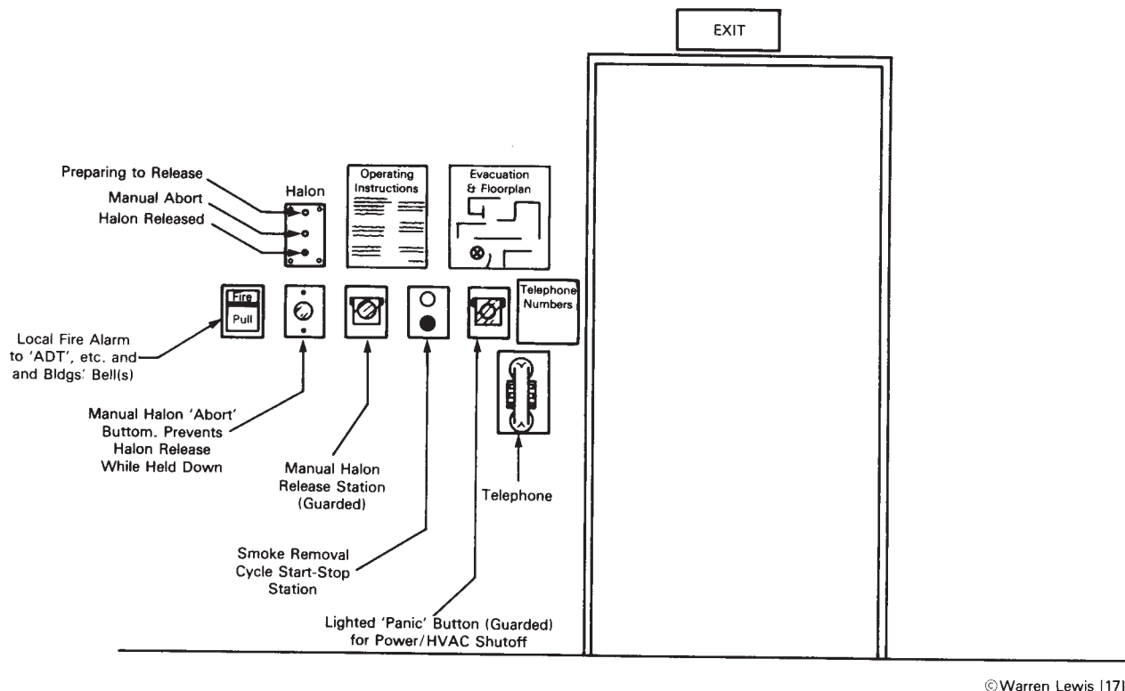
Figure 68. A well-organized, convenient, and coordinated arrangement of life-safety indicators and controls: An emergency telephone with separate line (not via PBX or switchboard) is needed near the exit and the life-safety indicators and controls. The audible alarm should not be so close to the telephone as to defeat attempts to communicate.
